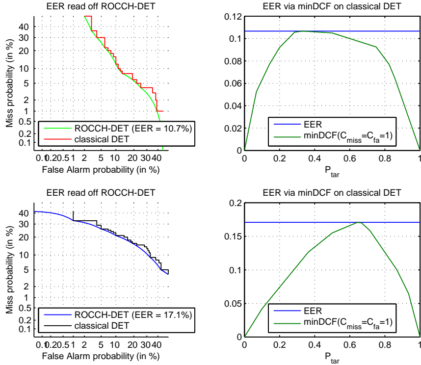
Figure 4: Two examples of ROCCH-DET vs classical steppy DET. The equality of ROCCH-EER and max minDCF is demonstrated. (Here \tilde{\pi} = P_{tar} ).
