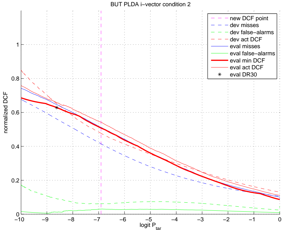
Figure 2: Normalized Bayes error-rate plot for an SRE 2010 speaker detector with good calibration. Here eval denotes the evaluation database and dev the development database. P_{\text{tar}} = \tilde{\pi} , while act DCF and min DCF refer to \mathcal{E} and \mathcal{E}_{\text{min}} . P_{\text{miss}} and normalized P_{\text{fa}} are shown separately. DR30 refers to the point to the left of which there are fewer than 30 false-alarms. The vertical magenta dashed line represents the new operating point at \tilde{\pi} = 0.001 .
