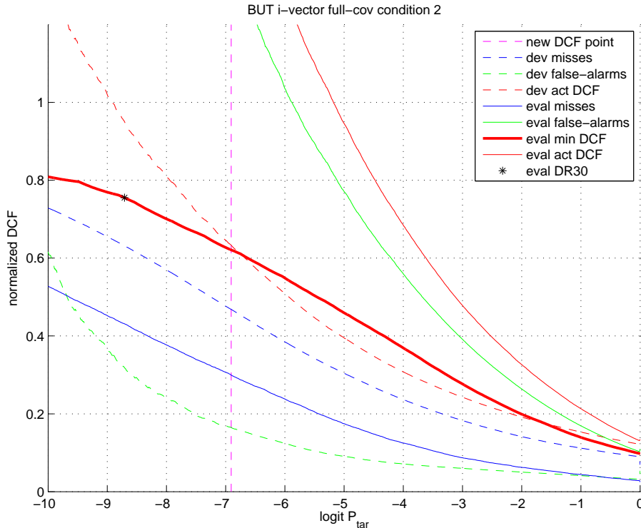
Figure 3: Normalized Bayes error-rate plot for an SRE 2010 speaker detector with bad calibration. See caption of figure 2 for details.
