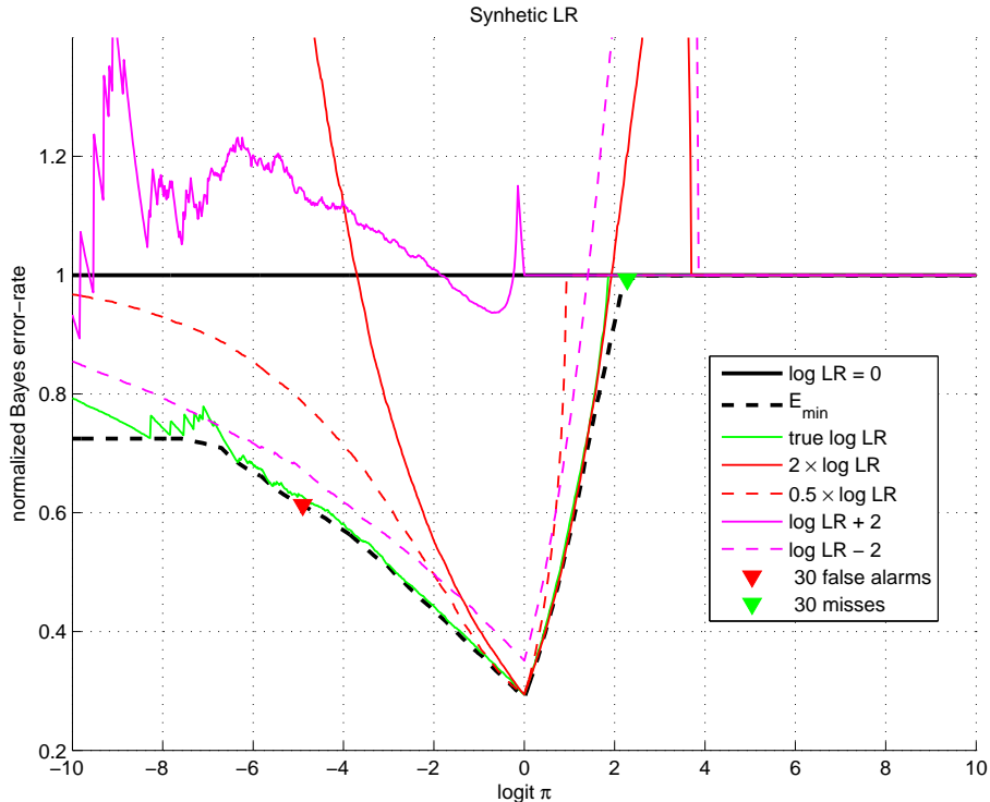
Figure 1: Normalized Bayes error-rate plot for a synthetic system with Gaussian scores: targets \sim \mathcal{N}(\mu = 3, \sigma = 2) and non-targets \sim \mathcal{N}(0, 1) . The true likelihood-ratio is compared against deliberate additive and multiplicative miscalibrations.
